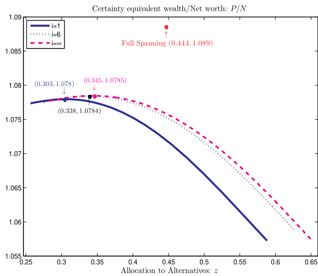
Figure 1. (Color online) Plot of P/N = p(w, t)/(w + 1) , the Ratio of the Certainty Equivalent Wealth P(W, K, t) = p(w, t)K and Net Worth N = W + K as a Function of the Portfolio's Percentage Allocation to Alternative Assets z = K/N
